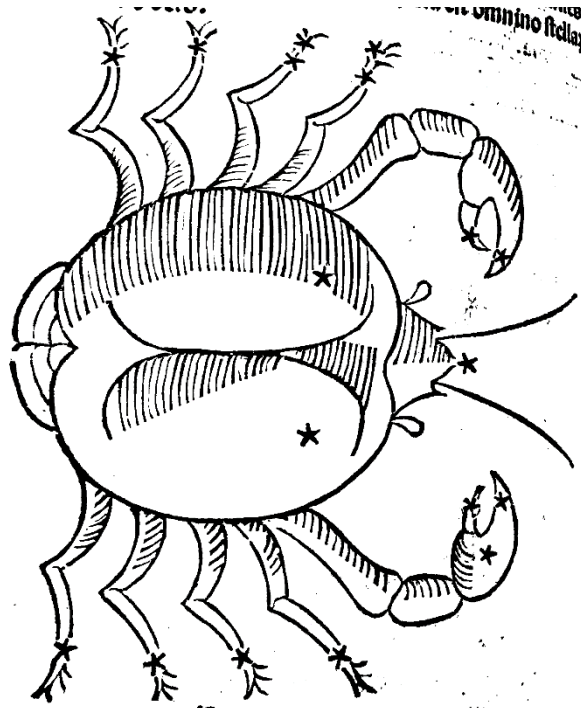
Cancer
