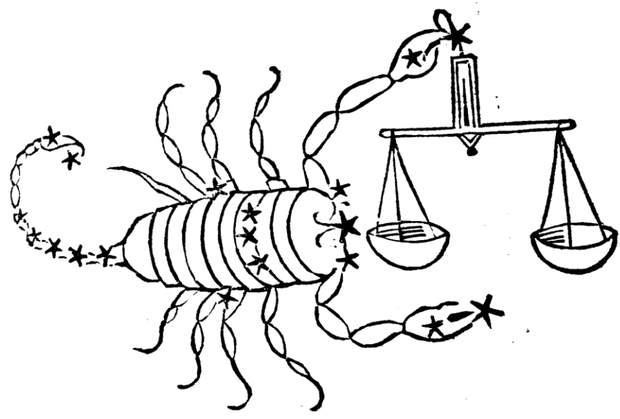
Scorpius
