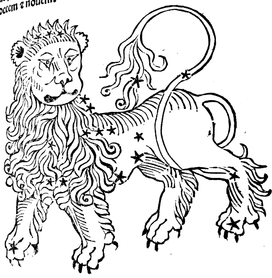
Leo
