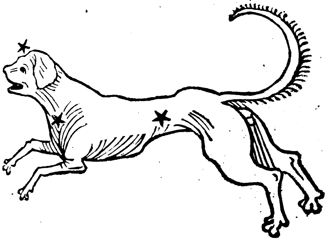
Canis minor
