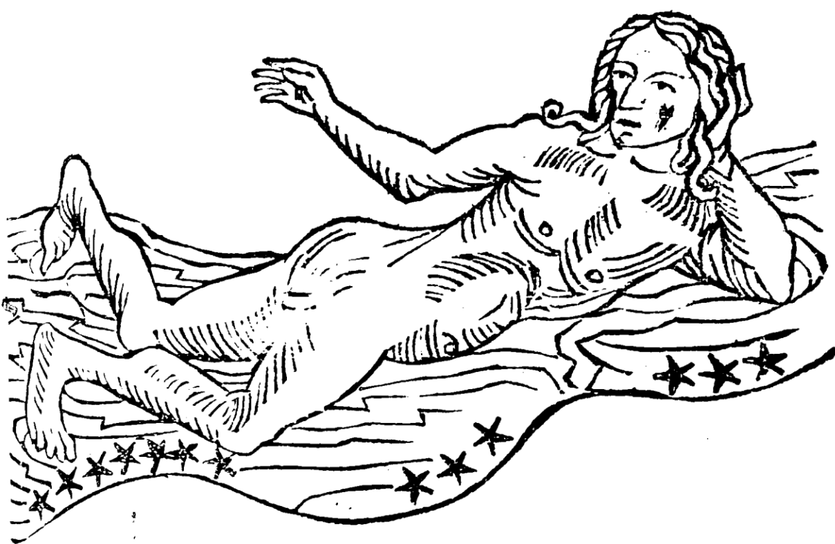
Eridanus flumen
